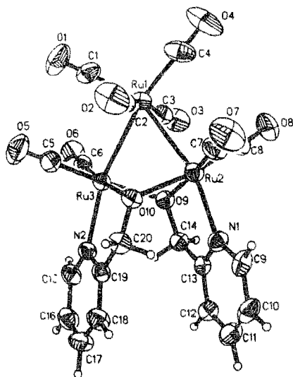
Fig. 5. Structure of \text{Ru}_3(\text{CO})_8(\mu\text{-}\eta^2\text{-OCH}_2\text{C}_5\text{H}_4\text{N})_2 . Reprinted with permission from Inorganic Chemistry . Copyright 1994 American Chemical Society.
