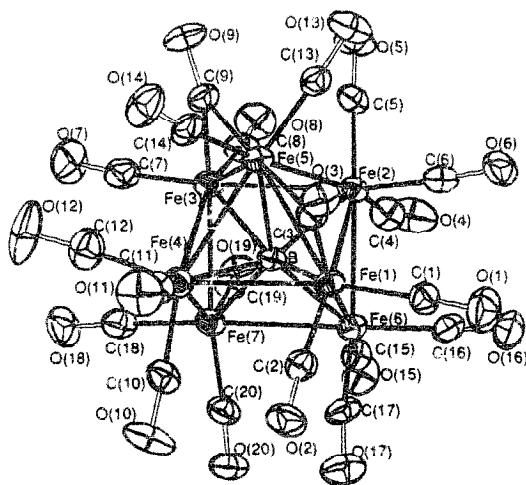
Fig. 15. Structure of [\text{HFe}_7(\text{CO})_{20}\text{B}]^{2-} . Reprinted with permission from Inorganic Chemistry. Copyright 1994 American Chemical Society.
