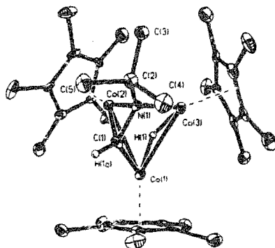
Fig. 17. Structure of Cp^*_3Co_3(\mu_3-\eta^2-CH=NBu^t)(\mu-H) . Reprinted with permission from Organometallics, Copyright 1994 American Chemical Society.
