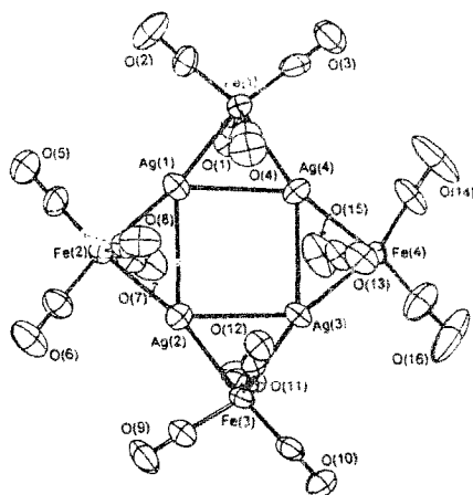
Fig. 28. Structure of [\text{Ag}_4\{\mu_2\text{-Fe}(\text{CO})_4\}_4]^{4-} . Reprinted with permission from Inorganic Chemistry. Copyright 1994 American Chemical Society.
