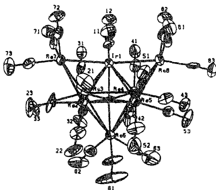
Fig. 27. Structure of [\text{Re}_7\text{IrC}(\text{CO})_{23}]^{2-} . Reprinted with permission from Journal of the American Chemical Society. Copyright 1994 American Chemical Society.
