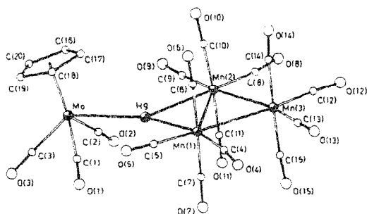
Fig. 25. Structure of [\text{Mn}_3(\text{CO})_{12}(\mu_3\text{-H})(\mu\text{-Hg})(\text{CpMo}(\text{CO})_3)] . Reprinted with permission from Organometallics. Copyright 1994 American Chemical Society.
