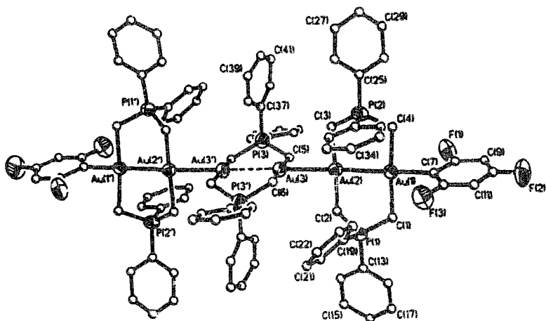
Fig. 18. Structure of [4\text{RAu}(\text{CH}_2\text{PPh}_2\text{CH}_2)_2\text{Au}]_2\text{Au}(\text{CH}_2\text{PPh}_2\text{CH}_2)_2\text{Au}]^+ ( \text{R} is \text{C}_6\text{H}_4\text{F}_3 ). Reprinted with permission from Organometallics. Copyright 1994 American Chemical Society.
