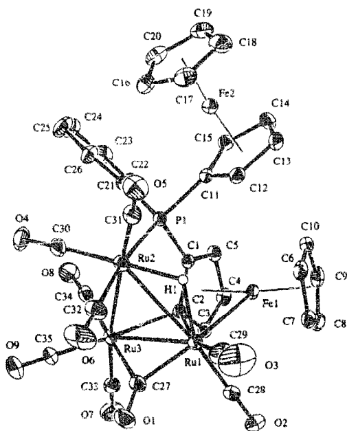
Fig. 6. Structure of \text{Ru}_3(\text{CO})_9(\mu\text{-CO})(\mu\text{-H})[\mu\text{-}\eta^3\text{-}\eta^5\text{-C}_6\text{H}_4\text{PFcPh}](\eta^5\text{-C}_5\text{H}_5) . Reprinted with permission from Organometallics . Copyright 1994 American Chemical Society.
