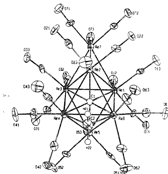
Fig. 2. Structure of the heptarhenium complex [\text{Re}_7\text{C}(\text{CO})_{21}(\mu\text{-H})_3] . Reprinted with permission from Organometallics. Copyright 1994 American Chemical Society.
