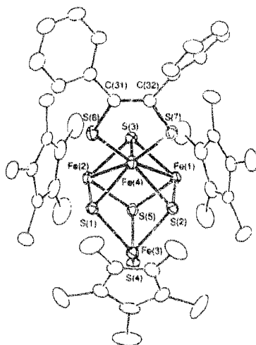
Fig. 11. Structure of \text{Cp}^*_3(\text{Ph}_2\text{C}_2\text{S}_2)_2\text{Fe}_4\text{S}_4 . Reprinted with permission from Inorganic Chemistry . Copyright 1994 American Chemical Society.
