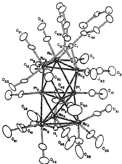
Fig. 26. Structure of \text{Ru}_6\text{Pt}_3(\text{CO})_{20}(\mu_3\text{-PhC}_2\text{Ph})(\mu_3\text{-H})(\mu\text{-H}) . Reprinted with permission from Organometallics. Copyright 1994 American Chemical Society.
