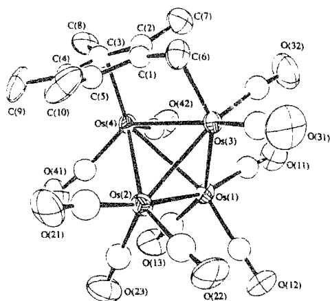
Fig. 12. Structure of [\mu,\eta^5,\eta^1\text{-C}_5\text{Me}_4\text{CH}_2]\text{Os}_4(\mu\text{-H})_2(\text{CO})_{10} . Reprinted with permission from Organometallics. Copyright 1994 American Chemical Society.
