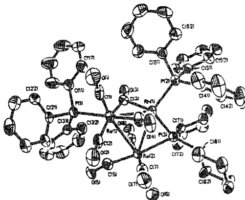
Fig. 20. Structure of \text{ReRh}(\mu\text{-CO})_2(\mu\text{-PR}_2)(\text{CO})_2(\text{PPh}_3)_2[\text{Re}(\text{CO})_4] . Reprinted with permission from Inorganic Chemistry. Copyright 1994 American Chemical Society.
