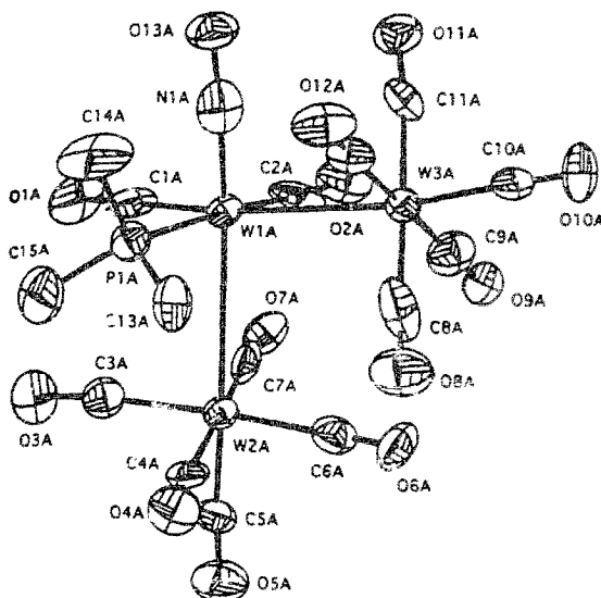
Fig. 1. Structure of the \text{PMe}_3 -substituted derivative of [\text{W}_3(\text{CO})_{13}(\text{NO})(\mu\text{-H})_2]^+ . Reprinted with permission from Inorganic Chemistry. Copyright 1994 American Chemical Society.
