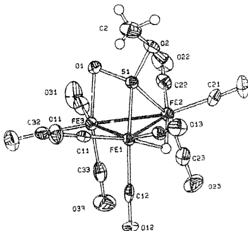
Fig. 7. Structure of \text{Fe}_3\text{CO}_9(\text{SO}_2\text{CH}_3)(\text{H}) . Reprinted with permission from Inorganic Chemistry . Copyright 1994 American Chemical Society.
