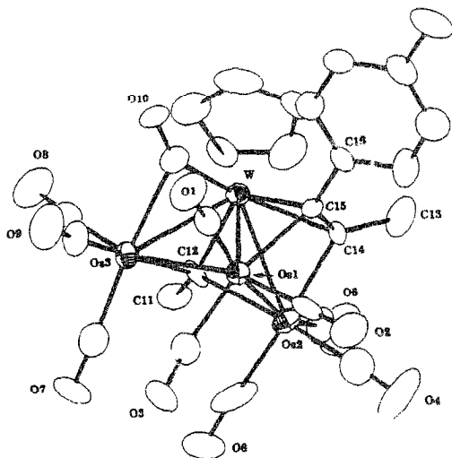
Fig. 22. Structure of \text{CpWOS}_3(\text{CO})_{10}(\mu_3\text{-C}_7\text{H}_7)(\text{C}_2\text{Me}_2) . Reprinted with permission from Organometallics . Copyright 1994 American Chemical Society.
