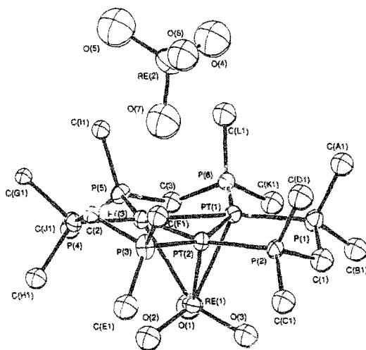
Fig. 23. Structure of [\text{Pt}_3(\text{ReO}_3)(\mu\text{-dppm})_3]^+ . Reprinted with permission from Journal of the American Chemical Society . Copyright 1994 American Chemical Society.
