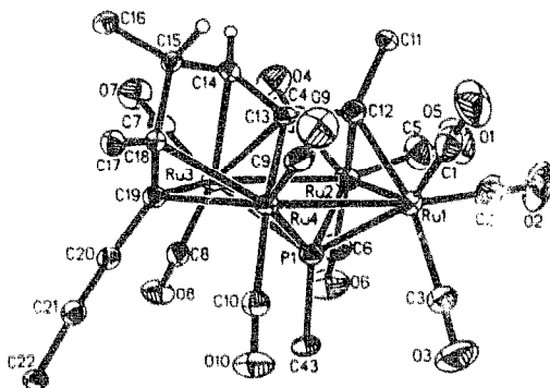
Fig. 10. Structure of \text{Ru}_4(\text{CO})_{10}(\mu_4\text{-PPh})[\mu_4\text{-}\eta^1\text{-}\eta^1\text{-}\eta^1\text{-}\eta^3\text{-PhCCC(H)C(H)PhC(Ph)CCCPh}] . Reprinted with permission from Organometallics. Copyright 1994 American Chemical Society.
