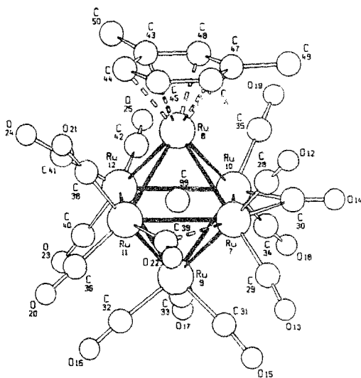
Fig. 14. Structure of \text{Ru}_6\text{C}(\text{CO})_{11}(\eta^6\text{-C}_6\text{H}_4\text{Me}_3)_7 . Reprinted with permission from Organometallics. Copyright 1994 American Chemical Society.
