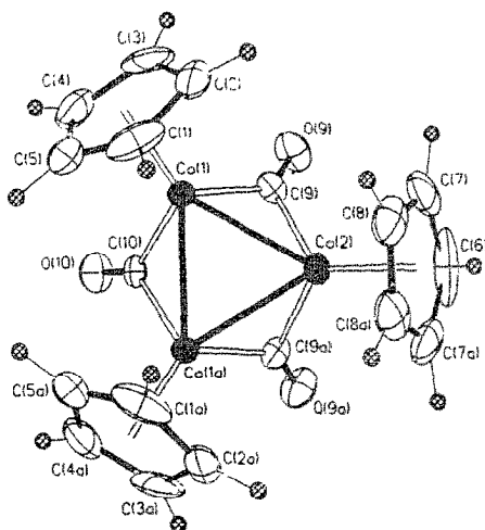
Fig. 16. Structure of \text{Cp}_3\text{Co}_3(\mu_2\text{-CO})_3 . Reprinted with permission from Inorganic Chemistry . Copyright 1994 American Chemical Society.
